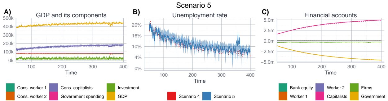
Figure 5: Model dynamics for scenario 5. The bold line represents the mean, the shaded area the inter-quartile range of the 15 simulation runs for scenario 5. The dashed lines refer to scenario 4 (see also Figure 4).
