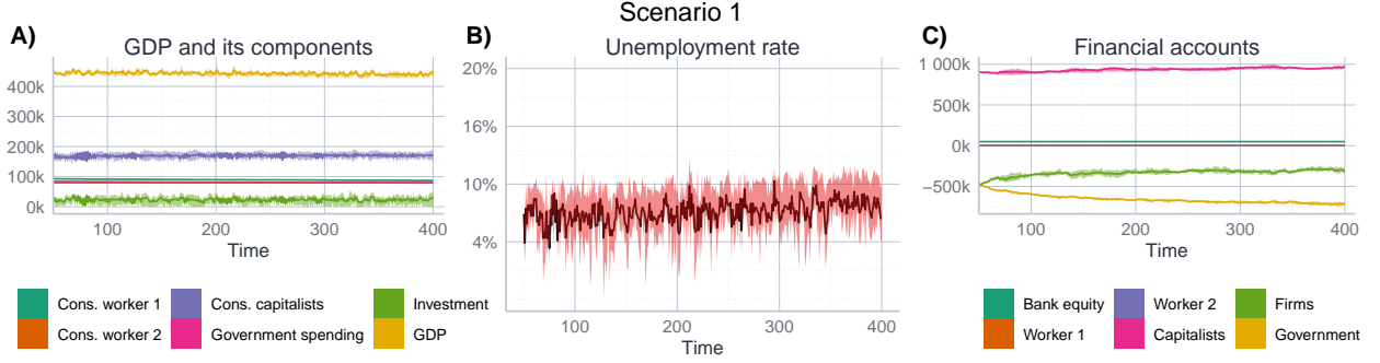
Figure 1: Model dynamics for scenario 1. The bold line represents the mean, the shaded area the inter-quartile range of the 15 simulation runs.
