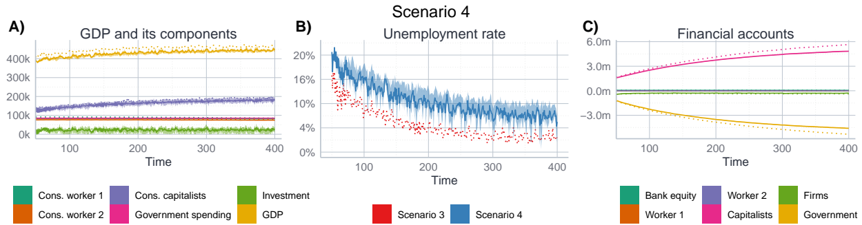
Figure 4: Model dynamics for scenario 4. The bold line represents the mean, the shaded area the inter-quartile range of the 15 simulation runs for scenario 4. The dashed lines refer to scenario 3 (see also Figure 3).
