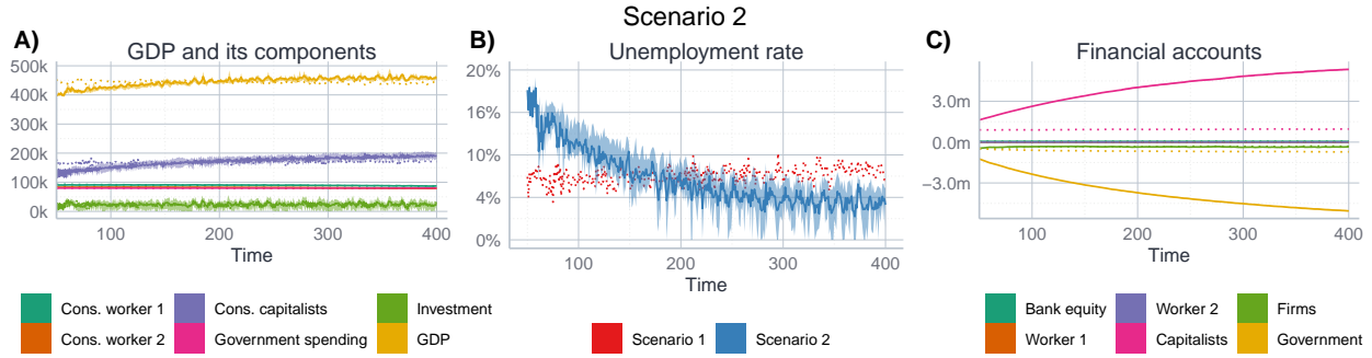
Figure 2: Model dynamics for scenario 2. The bold line represents the mean, the shaded area the inter-quartile range of the 15 simulation runs for scenario 2. The dashed lines refer to scenario 1 (see also Figure 1).
